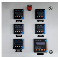
PID Controllers, Temperature Indicators, Data Recorder in MS Powder Coated Panel
